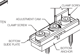
BOTTOM PIVOT ADJUSTMENT
